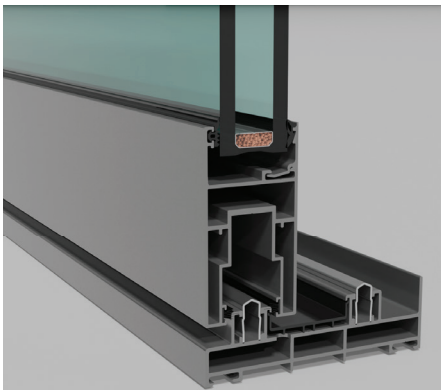
Bottom detail_normal threshold
